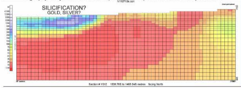
These sections indicate two possible modes of gold mineralization that represent the geophysical extremes included within a fs3D data based inversion model, - the unmistakable high-ratio anomaly below, and, above, the subtle patterns from which a geophysically-invisible structure (a deep feeder) can be inferred and positioned.
