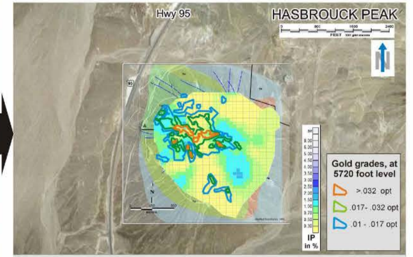
3D IP reveals no significant chargeability anomalies. Typical values are less than 1.5%, nominally "background".
